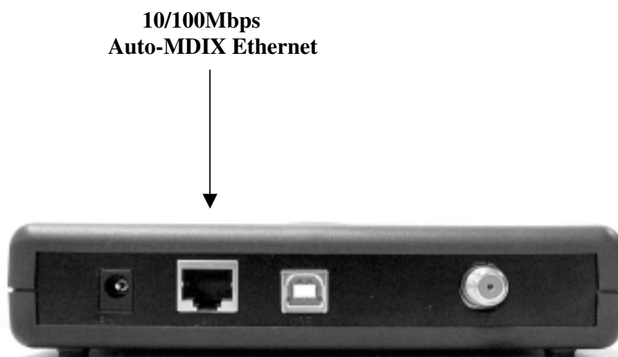
Figure 3a. Connecting to a Network Interface Card
